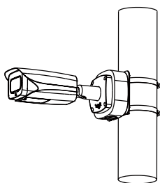
PFA121+PFA152 Pole Mount
